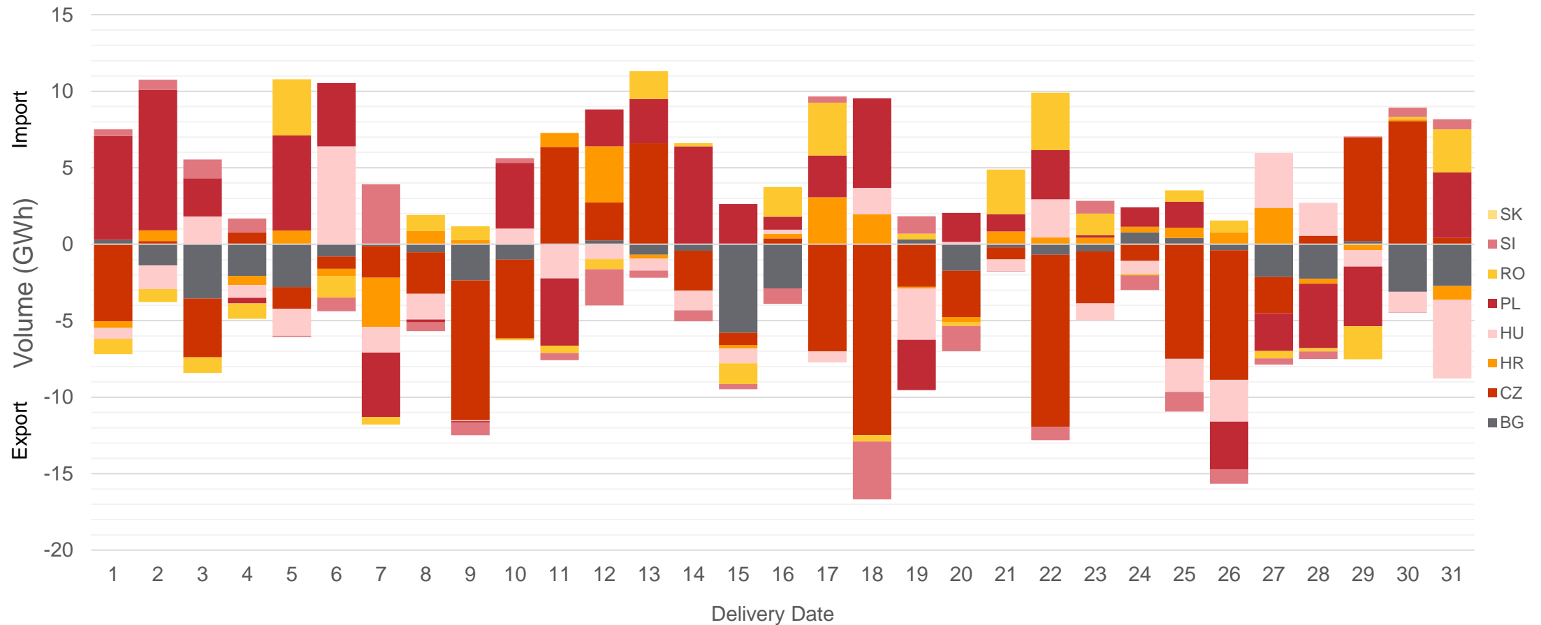
2021-3 Intraday Net Positions CEE+SEE
