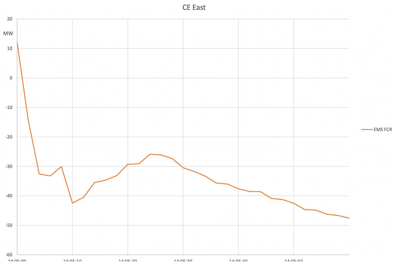
Figure A2-53: EMS FCR
