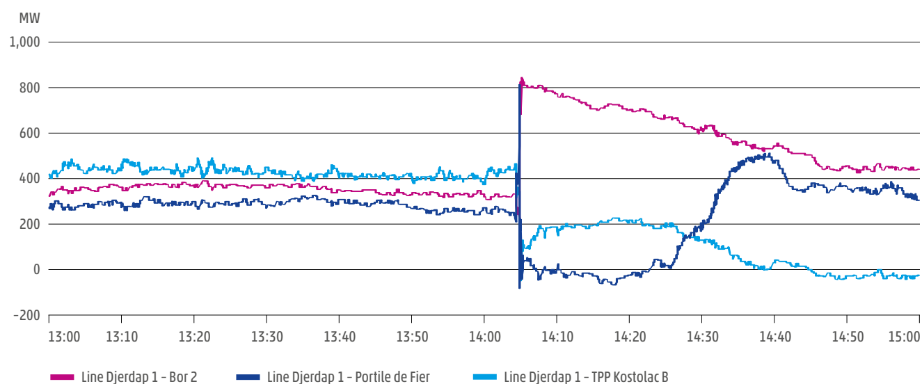
Figure A1-3: Power flows through the individual elements connected to busbars in SS Đerdap 1
