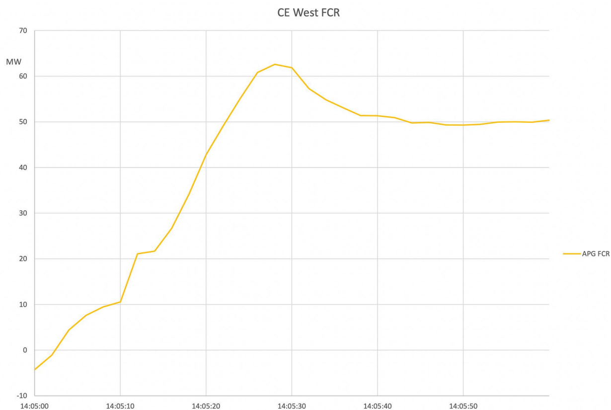
Figure A2-7: APG FCR
