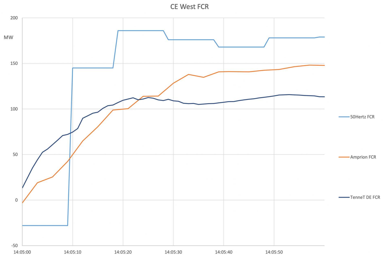
Figure A2-3: DE FCR
