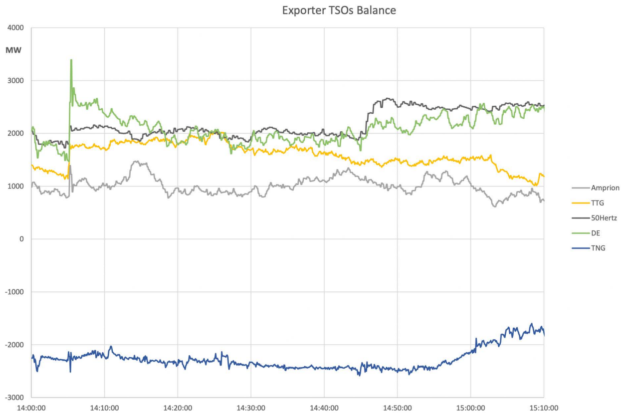
Figure A2-2: DE Balance
