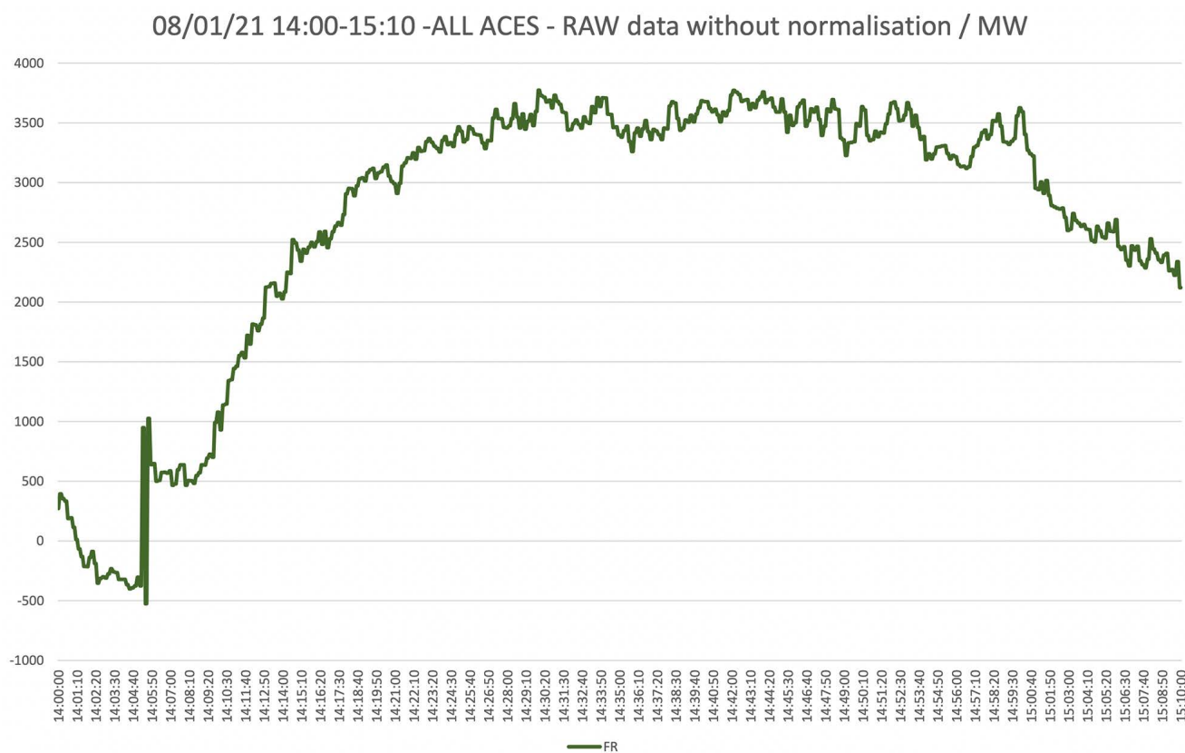
Figure A2-33: RTE ACE
