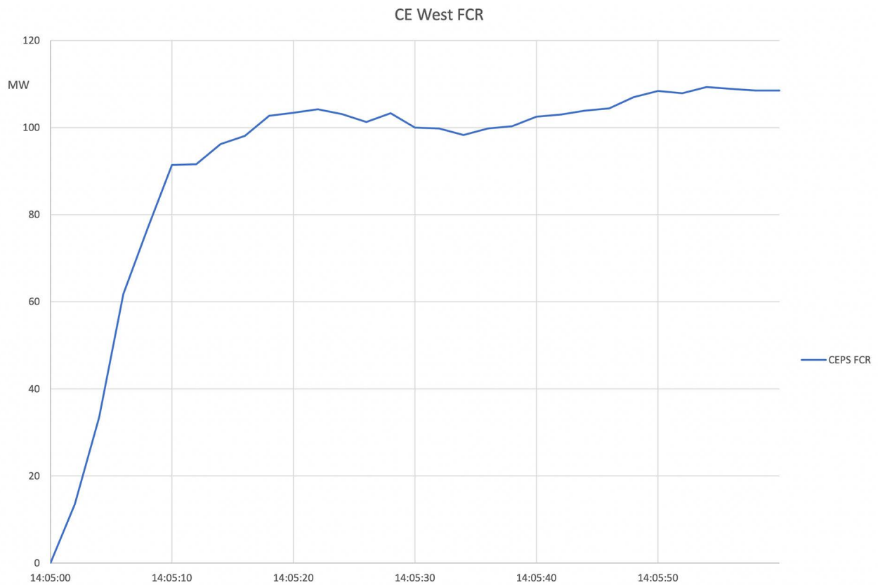
Figure A2-10: CEPS FCR
