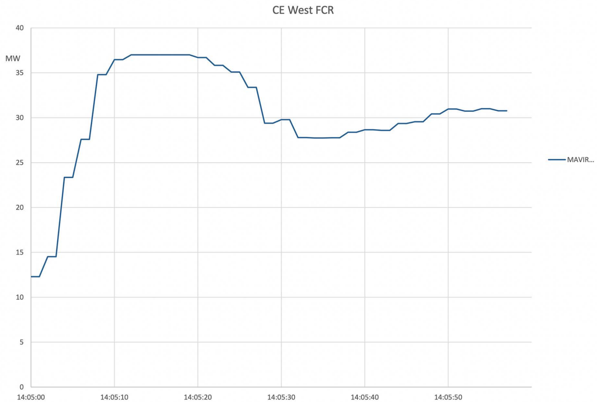
Figure A2-24: Mavir FCR
