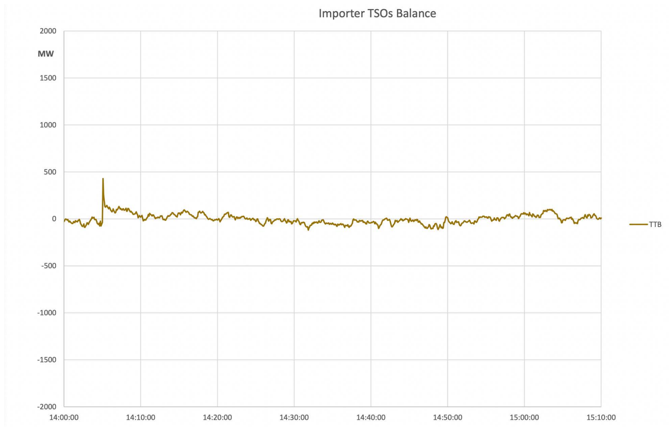
Figure A2-42: TenneT NL Balance
