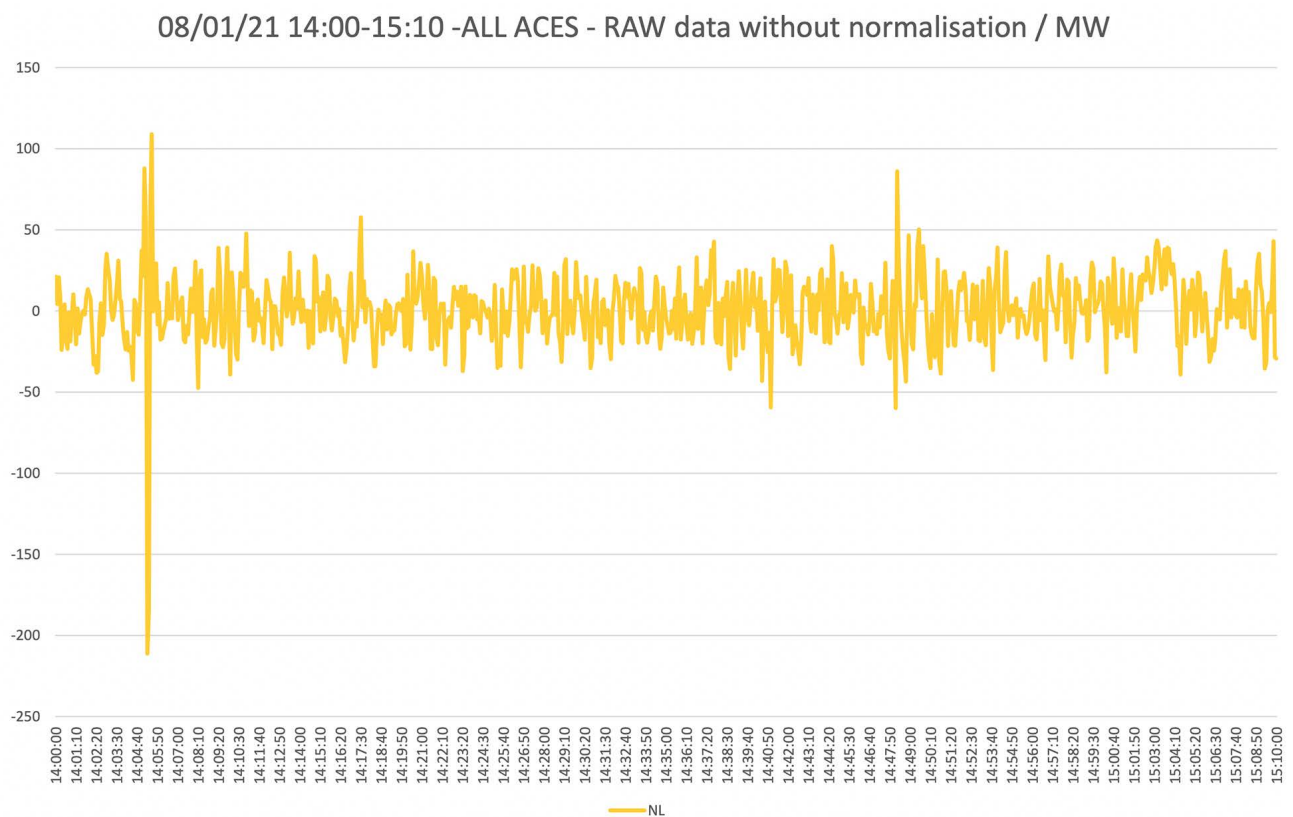
Figure A2-41: TenneT NL ACE
