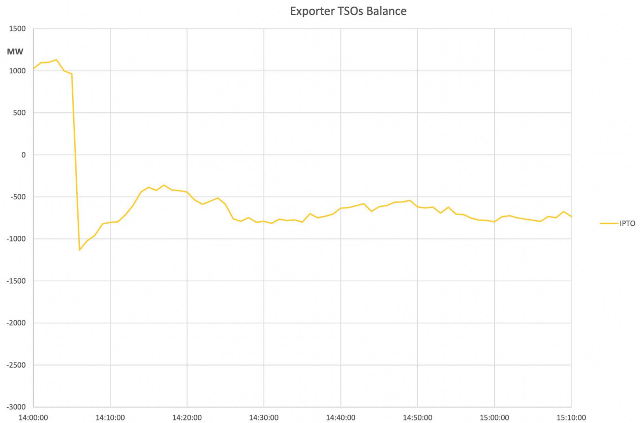
Figure A2-58: IPTO Balance
