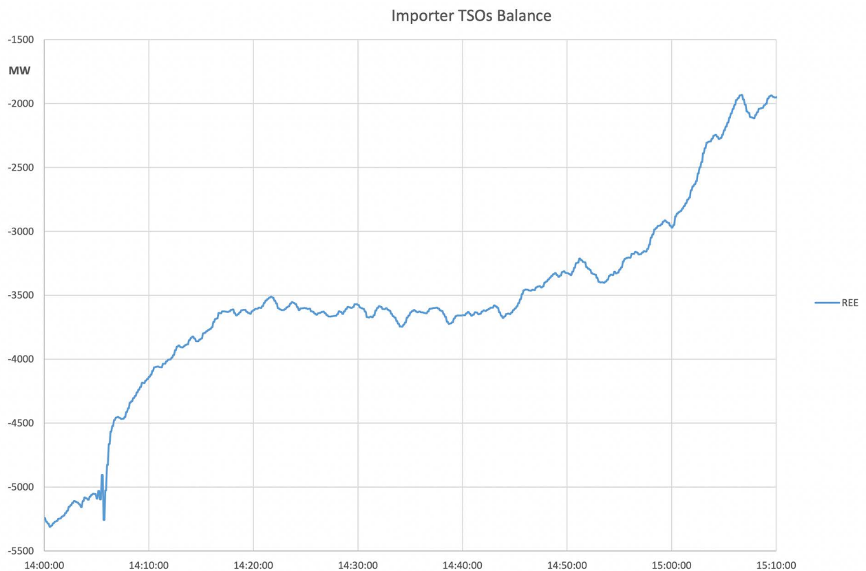
Figure A2-29: REE Balance
