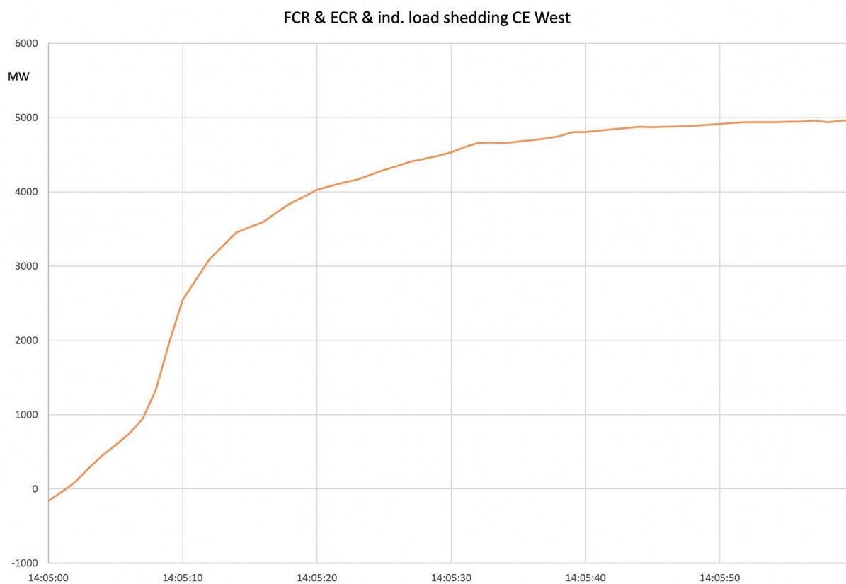
Figure A2-47: CE West Sum of FCR & EPC & SPS
