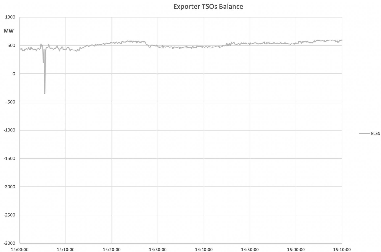
Figure A2-12: ELES Balance
