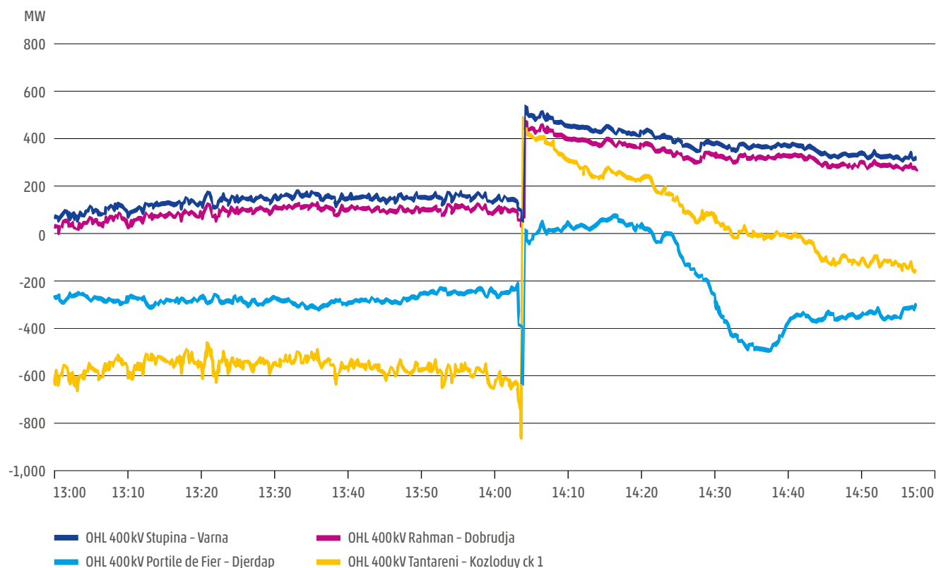
Figure A1-4: Power flows through the Romanian tie-lines within the South-East split area
