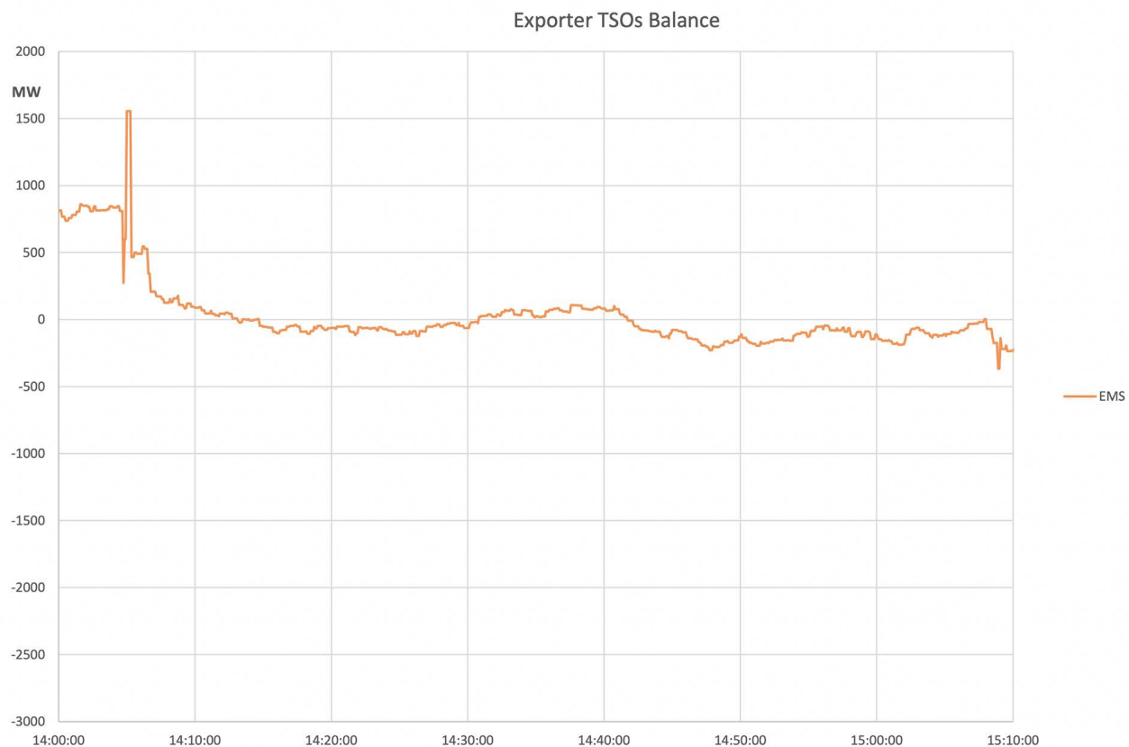
Figure A2-52: EMS Balance
