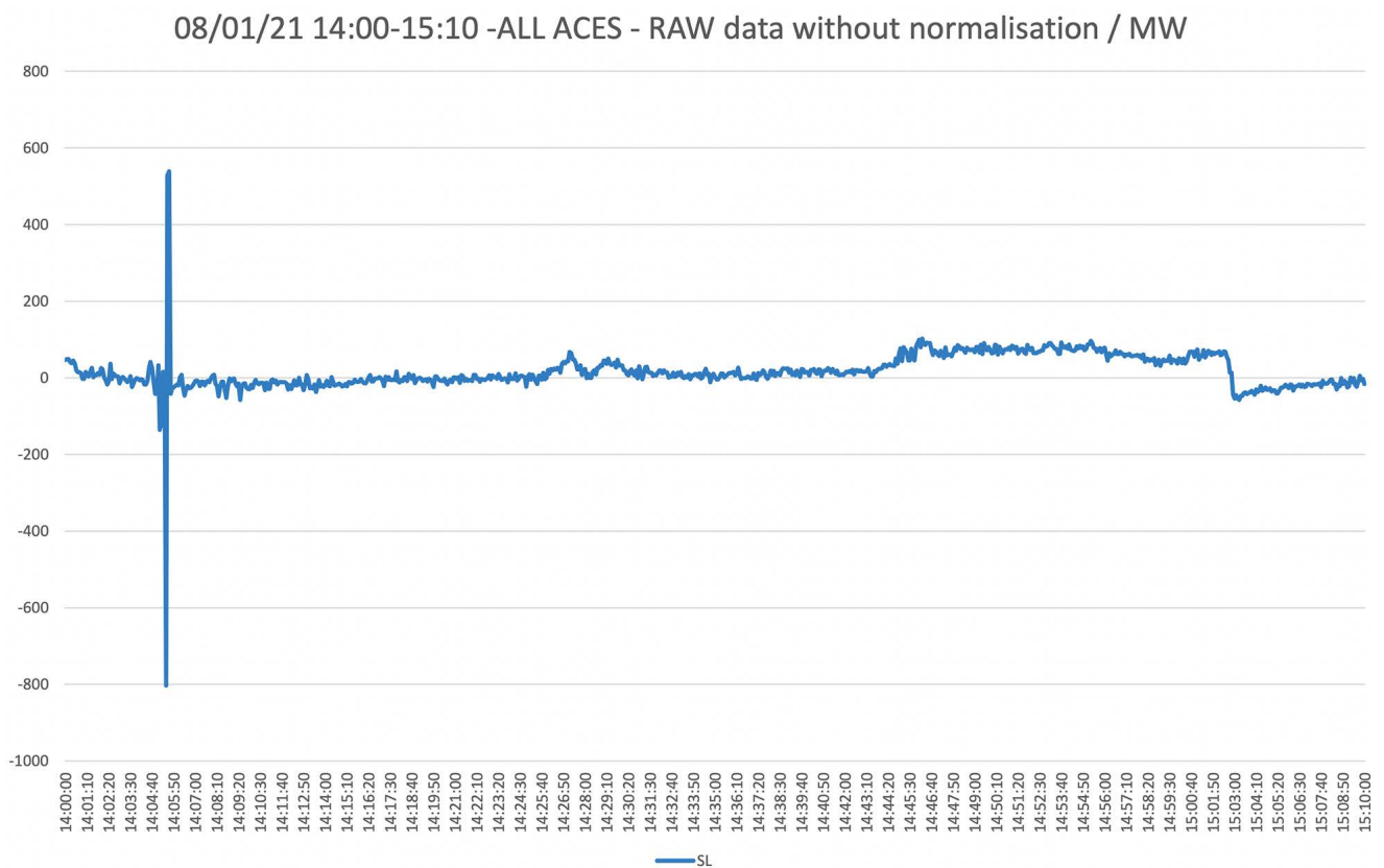
Figure A2-11: ELES ACE
