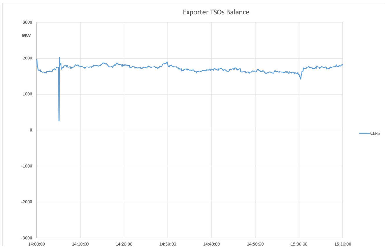
Figure A2-9: CEPS Balance
