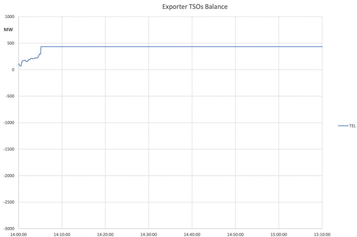
Figure A2-70: Transelectrica Balance
