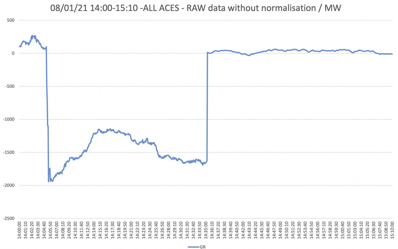
Figure A2-57: IPTO ACE
