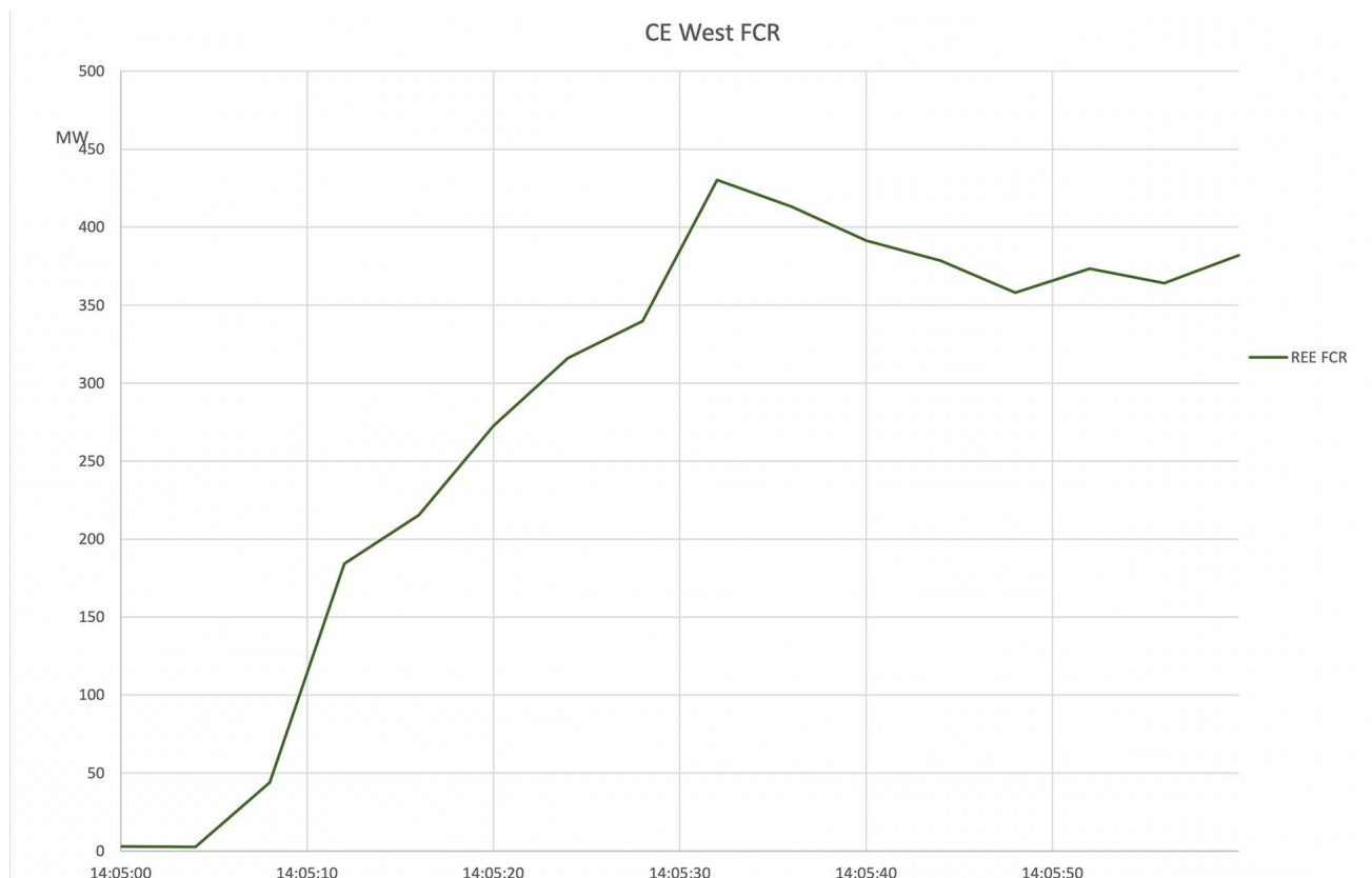
Figure A2-30: REE FCR
