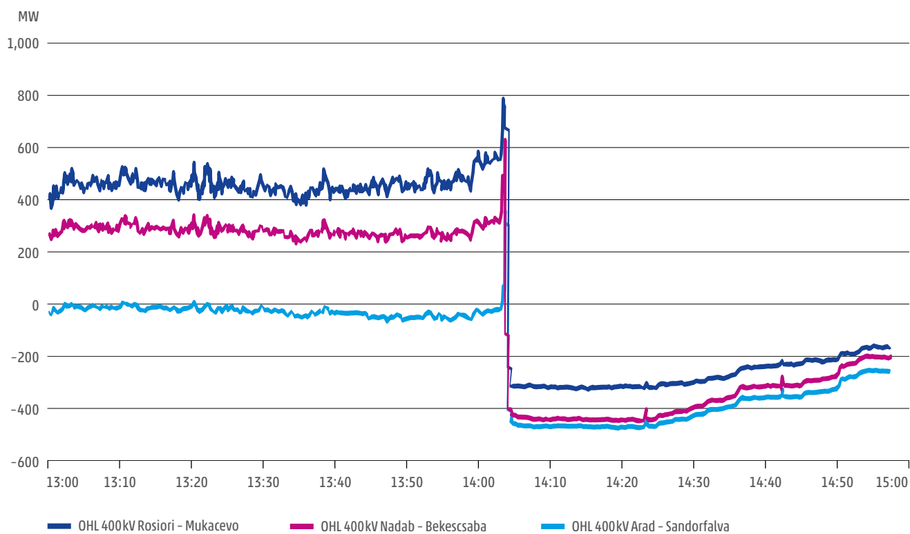
Figure A1-5: Power flows through the Romanian tie-lines within the North-West area
