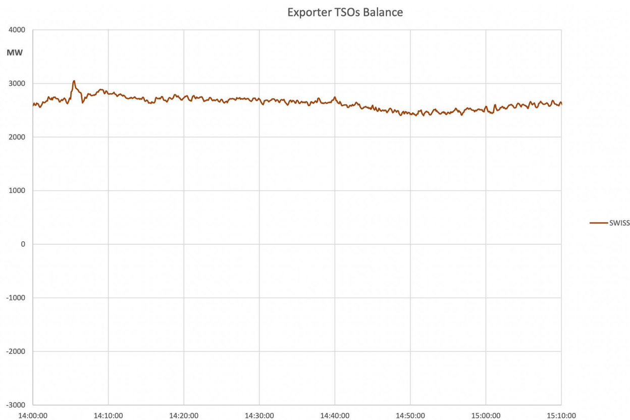
Figure A2-39: Swissgrid Balance
