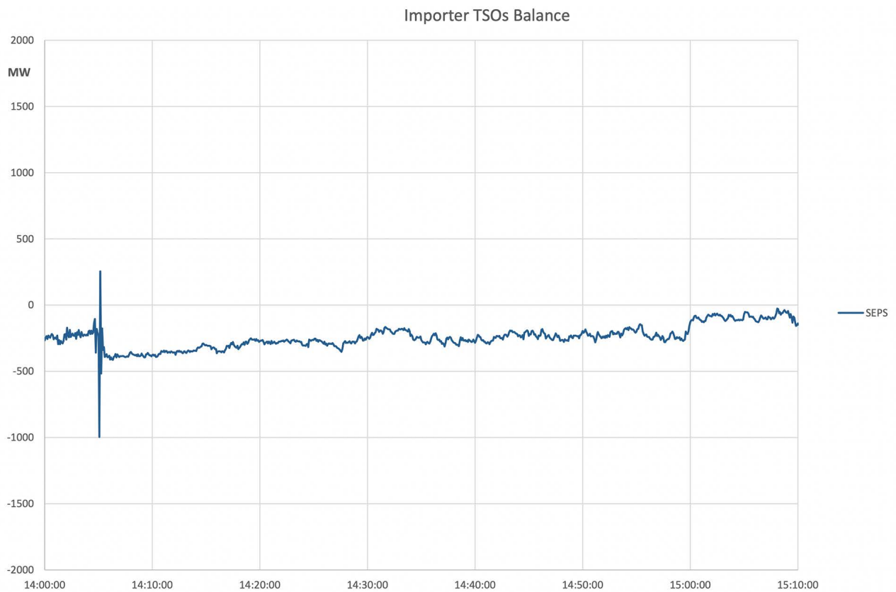
Figure A2-37: SEPS Balance
