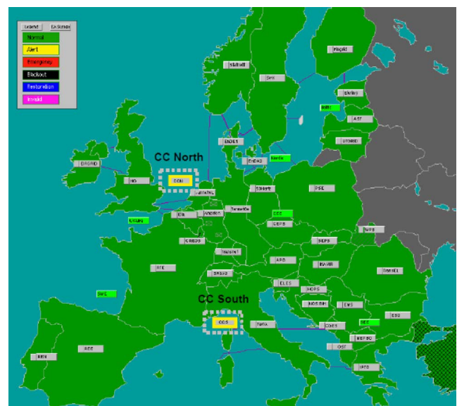
Figure 1.1: EAS frequency state traffic lights with status "yellow"
