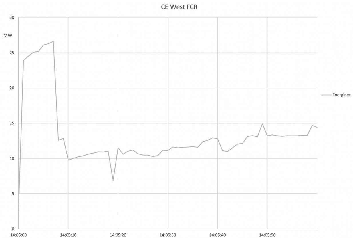
Figure A2-19: Energinet FCR
