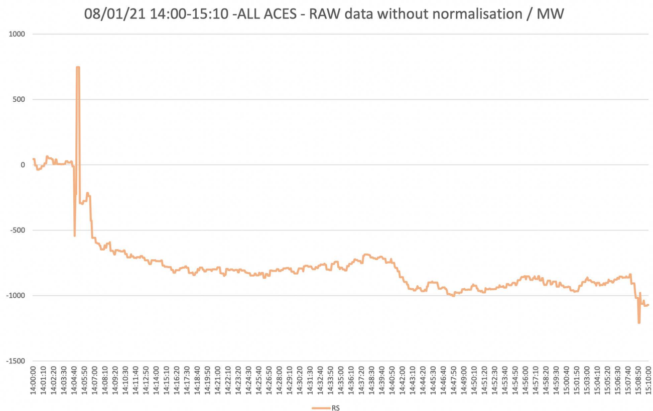
Figure A2-51: EMSACE
