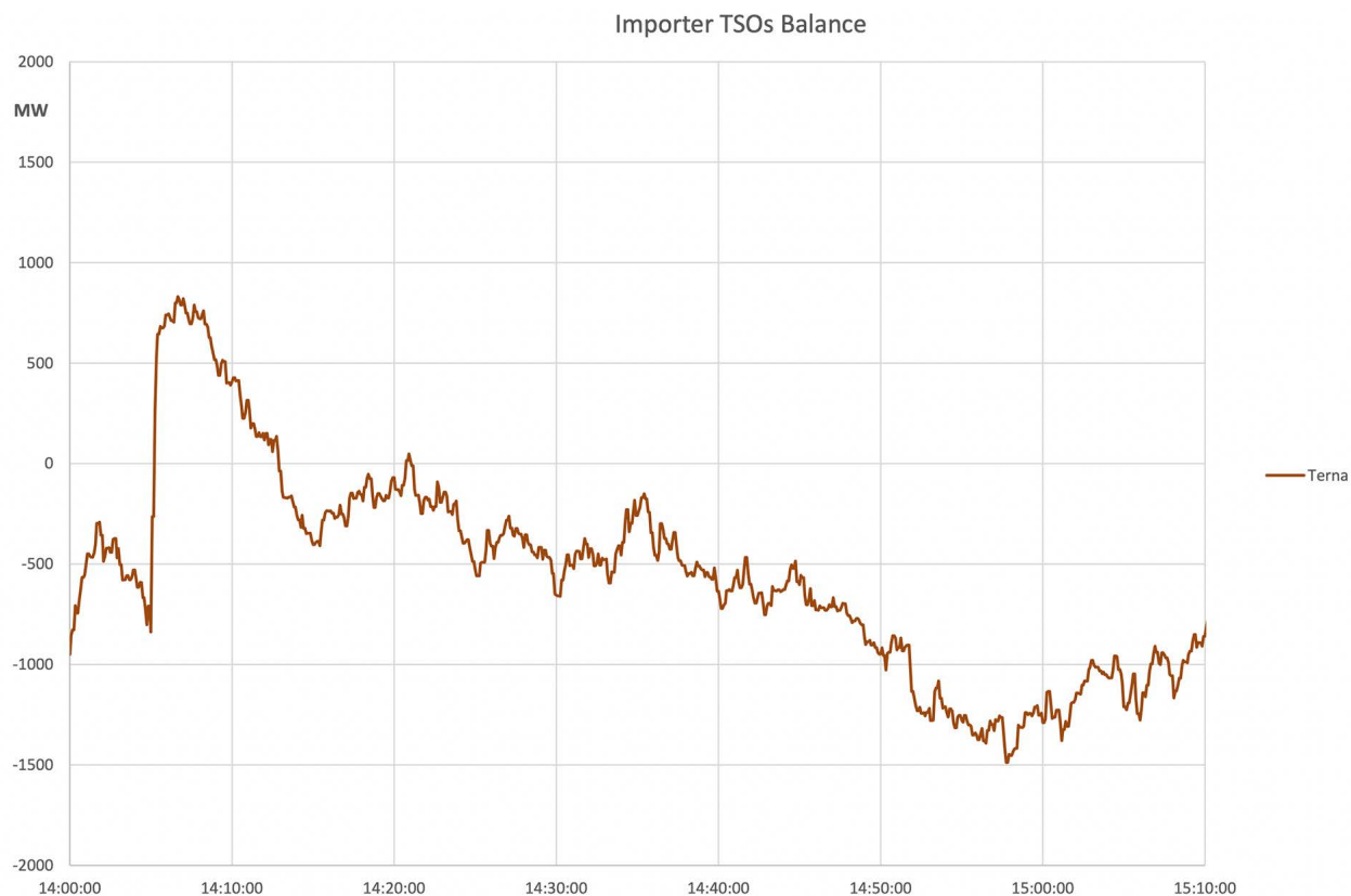
Figure A2-45: Terna Balance
