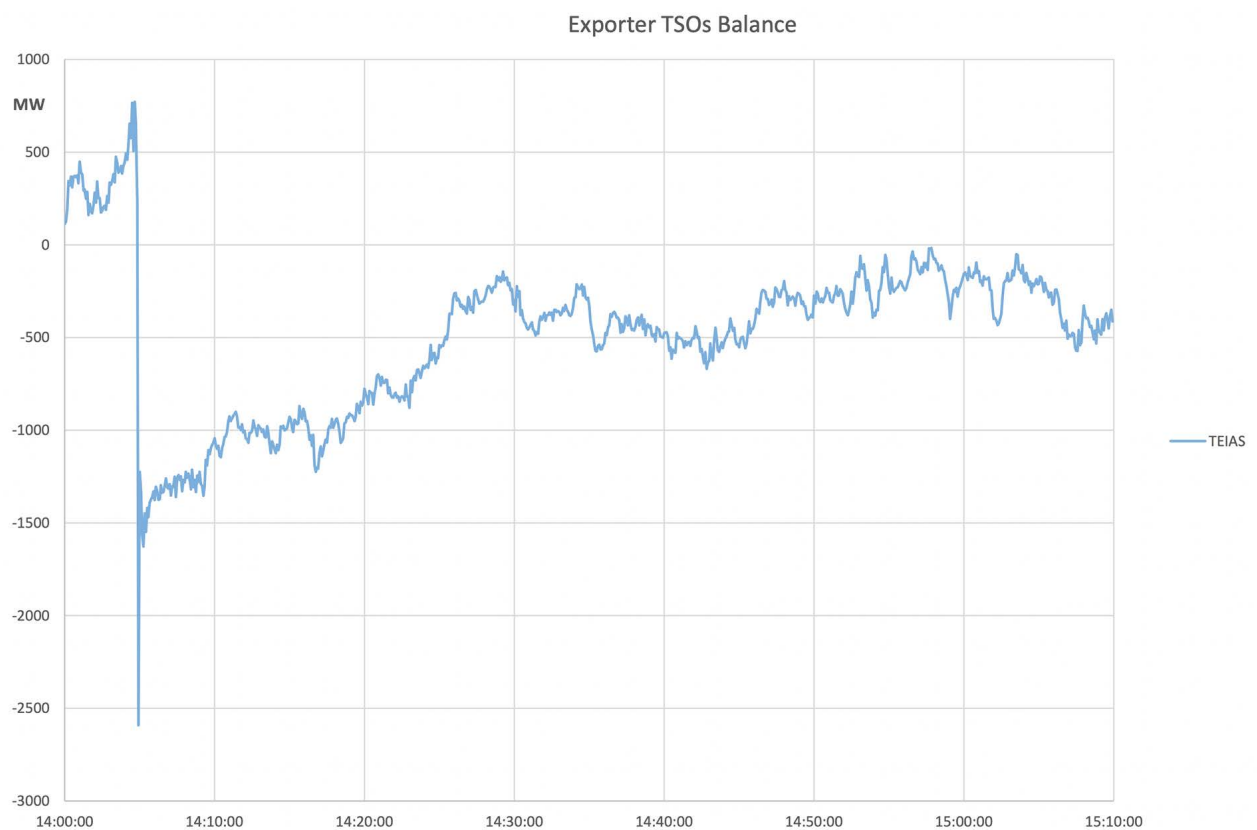
Figure A2-67: TEIAS Balance
