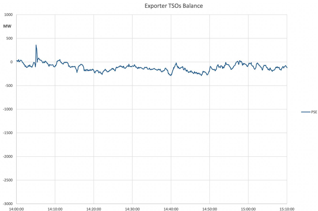
Figure A2-26: PSE Balance
