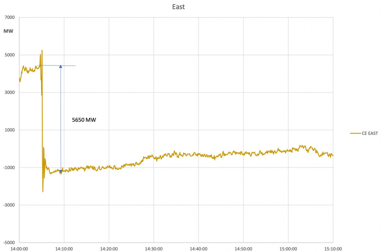
Figure A2-73: Balance CE East Sum
