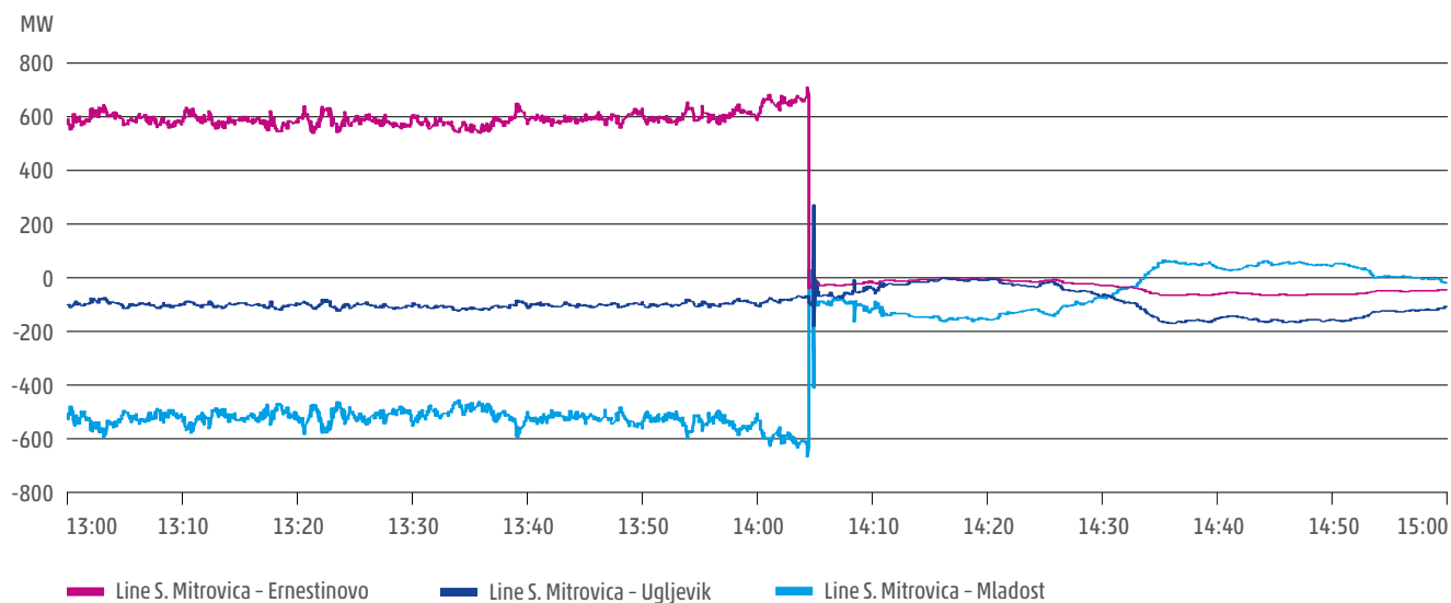
Figure A1-1: Power flows through the individual elements connected to busbars in SS Sremska Mitrovica 2
