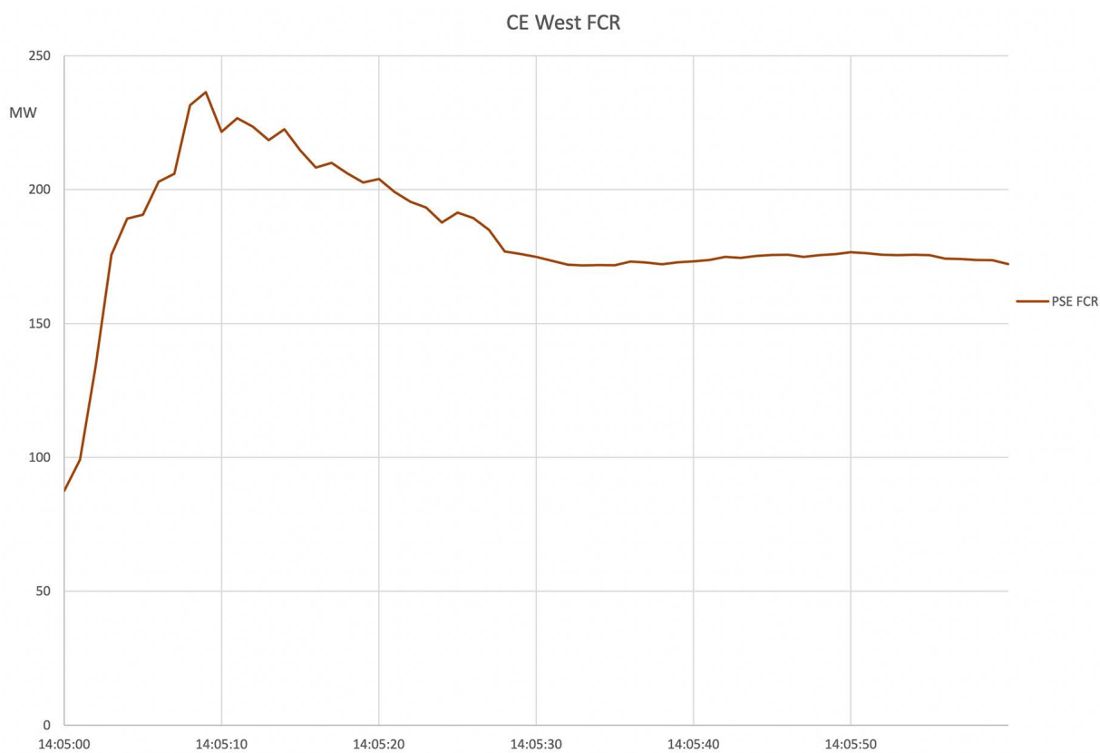
Figure A2-27: PSE FCR
