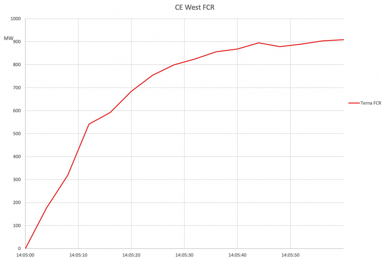
Figure A2-46: Terna FCR
