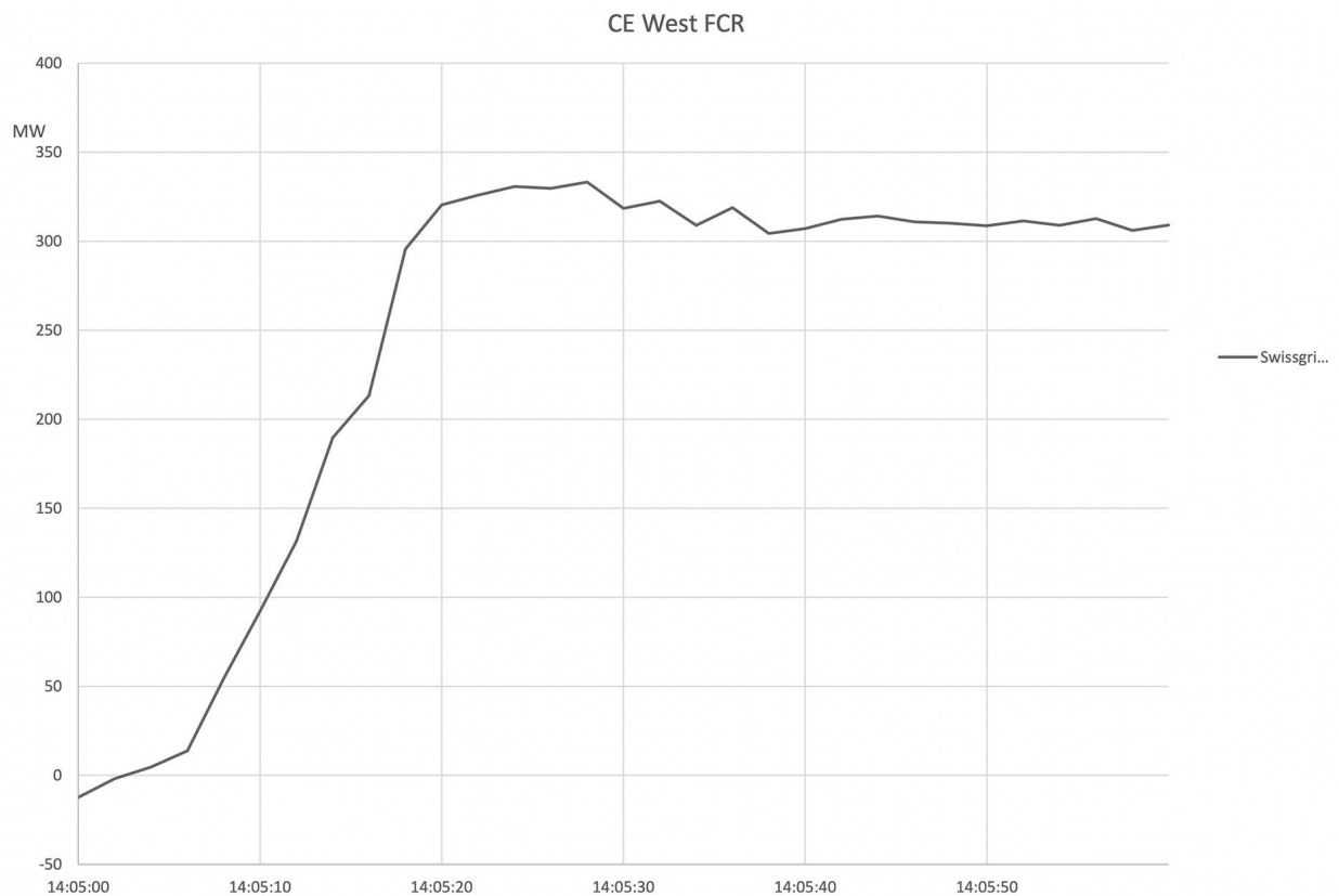
Figure A2-40: Swissgrid FCR
