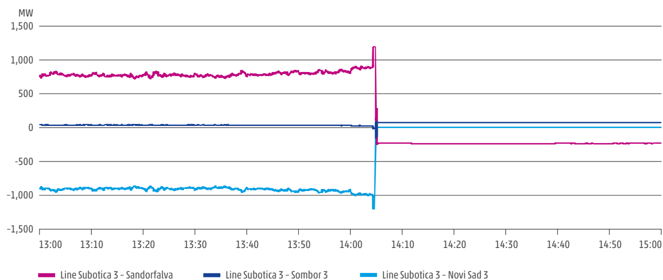
Figure A1-2: Power flows through the individual elements connected to busbars in SS Subotica
