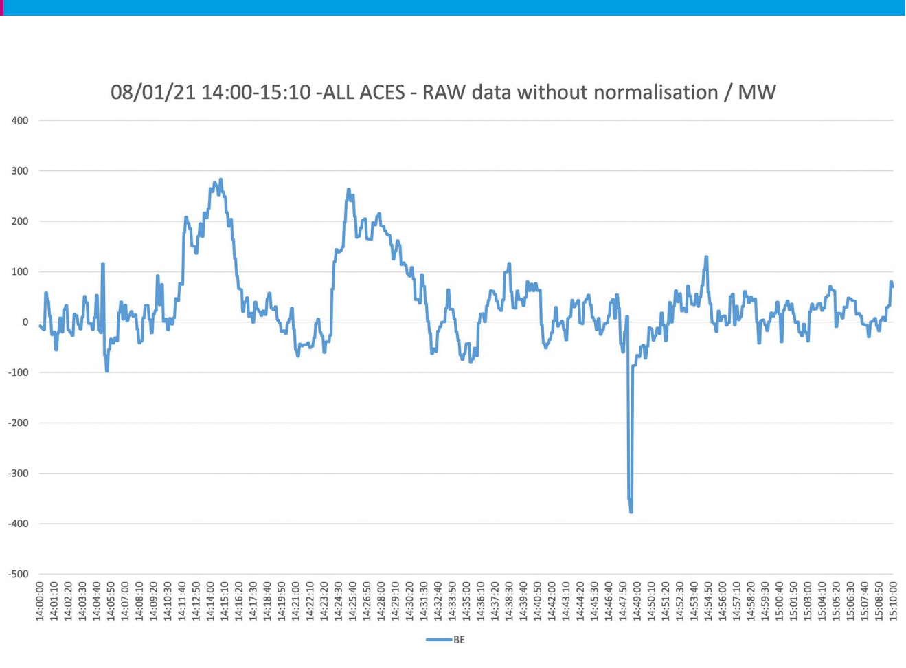
Figure A2-14: ELIA ACE
