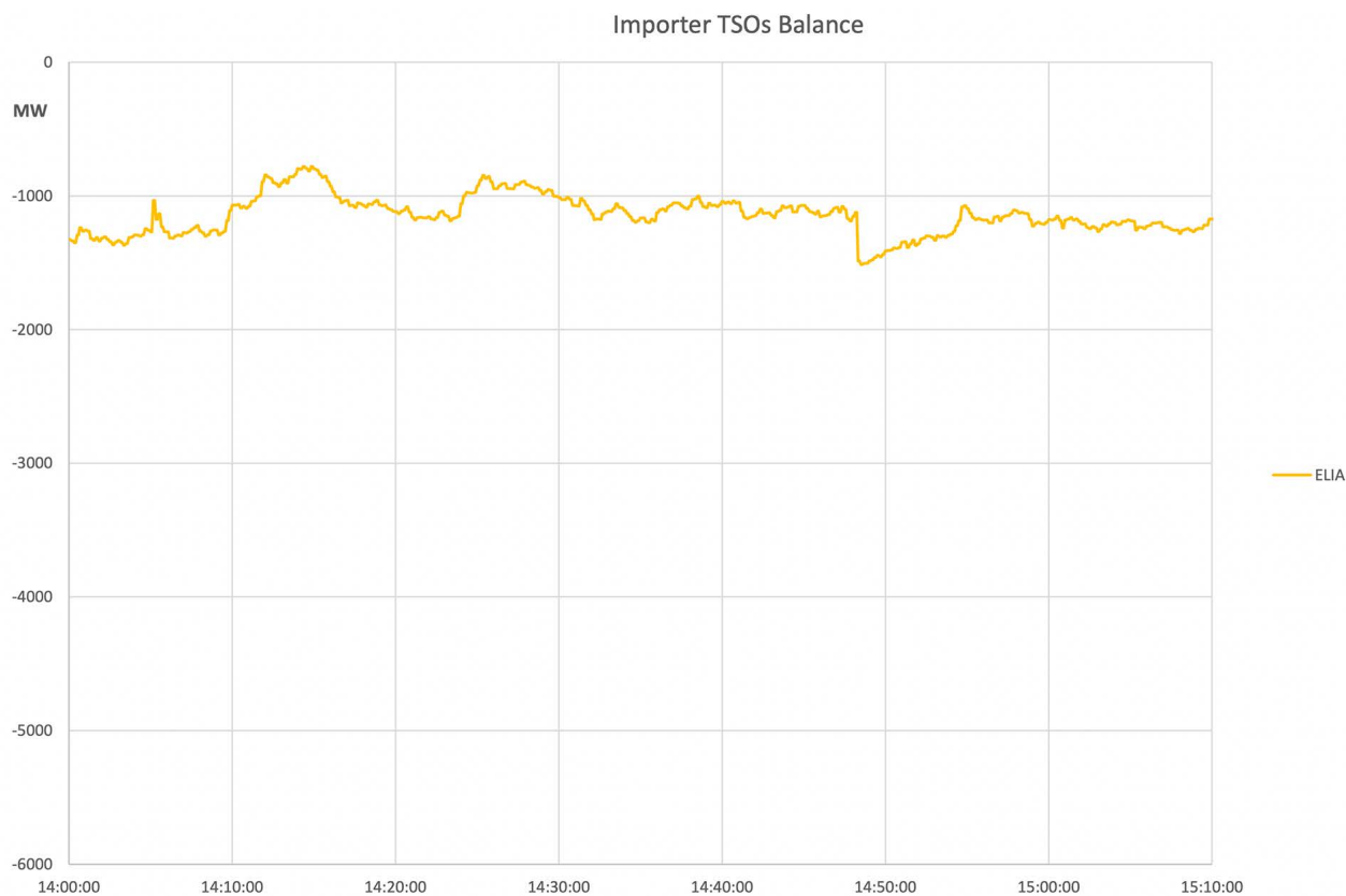
Figure A2-15: ELIA Balance
