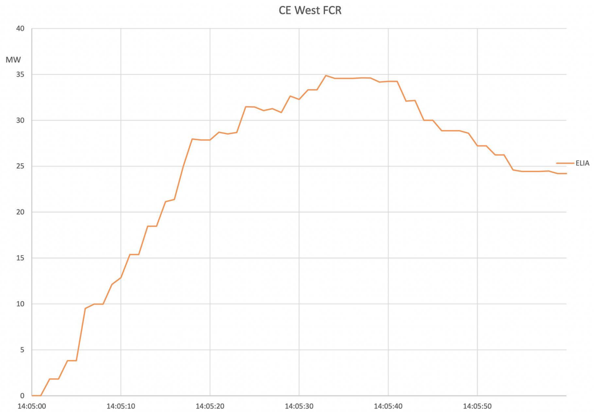
Figure A2-16: ELIA FCR
