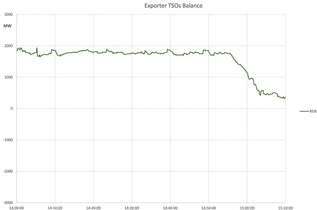
Figure A2-32: REN Balance
