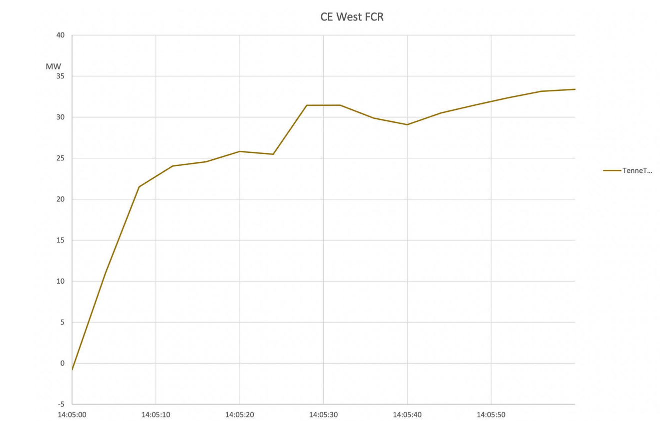
Figure A2-43: TenneT NL FCR
