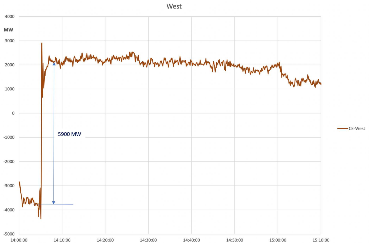
Figure A2-72: Balance CE West Sum
