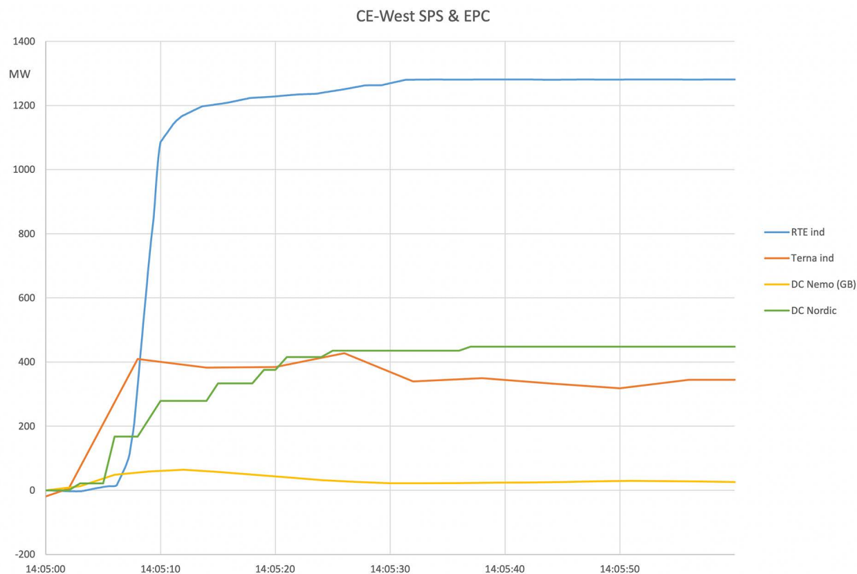
Figure A2-4: EPC and SPS Support
