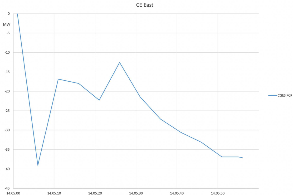
Figure A2-50: CGES FCR
