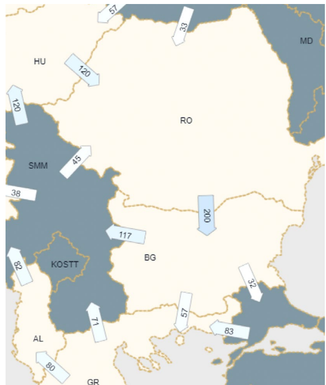
Figure 54: Average PTDF Flow Indicator for 2019 (in MW) – CCR: Southeast Europe (SEE)
