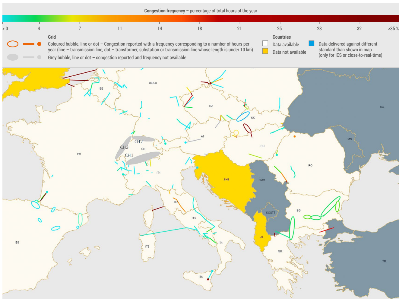
Figure 77: CCDA for 2019 – Balkans and Italy without threshold
