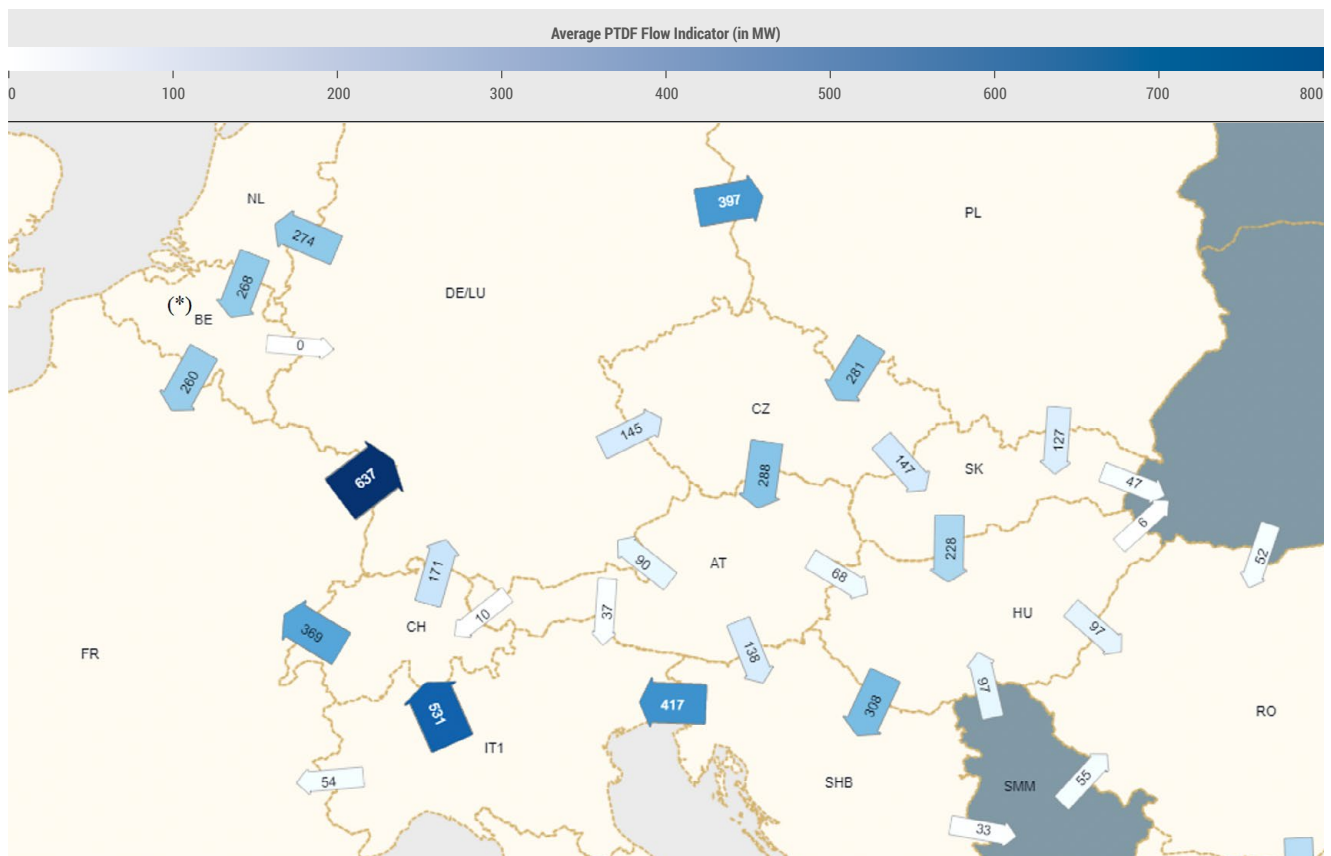
Figure 52: Average PTDF Flow Indicator for 2020 (in MW). CCR: Core and Italy North (CH-FR, CH-IT, CH-DE/LU, CH-AT, UA-SK, UA-HU, UA-RO bidding zone borders are not part of these CCRs). *Please note that in the context of the minimum 70 % requirement set by Regulation 2019/943, Elia and TenneT TSO B.V. obtained a derogation for excessive loopflows. The methodology for calculation of the loopflows is described in the respective derogations granted to Elia and TenneT TSO B.V. and differs from the methodology applied in this report, the key difference being that the loopflows are calculated using the CWE FB DA CC parameters and thus D2CF data. The result of these loopflow calculations is reported through the JAO Utility Tool.
