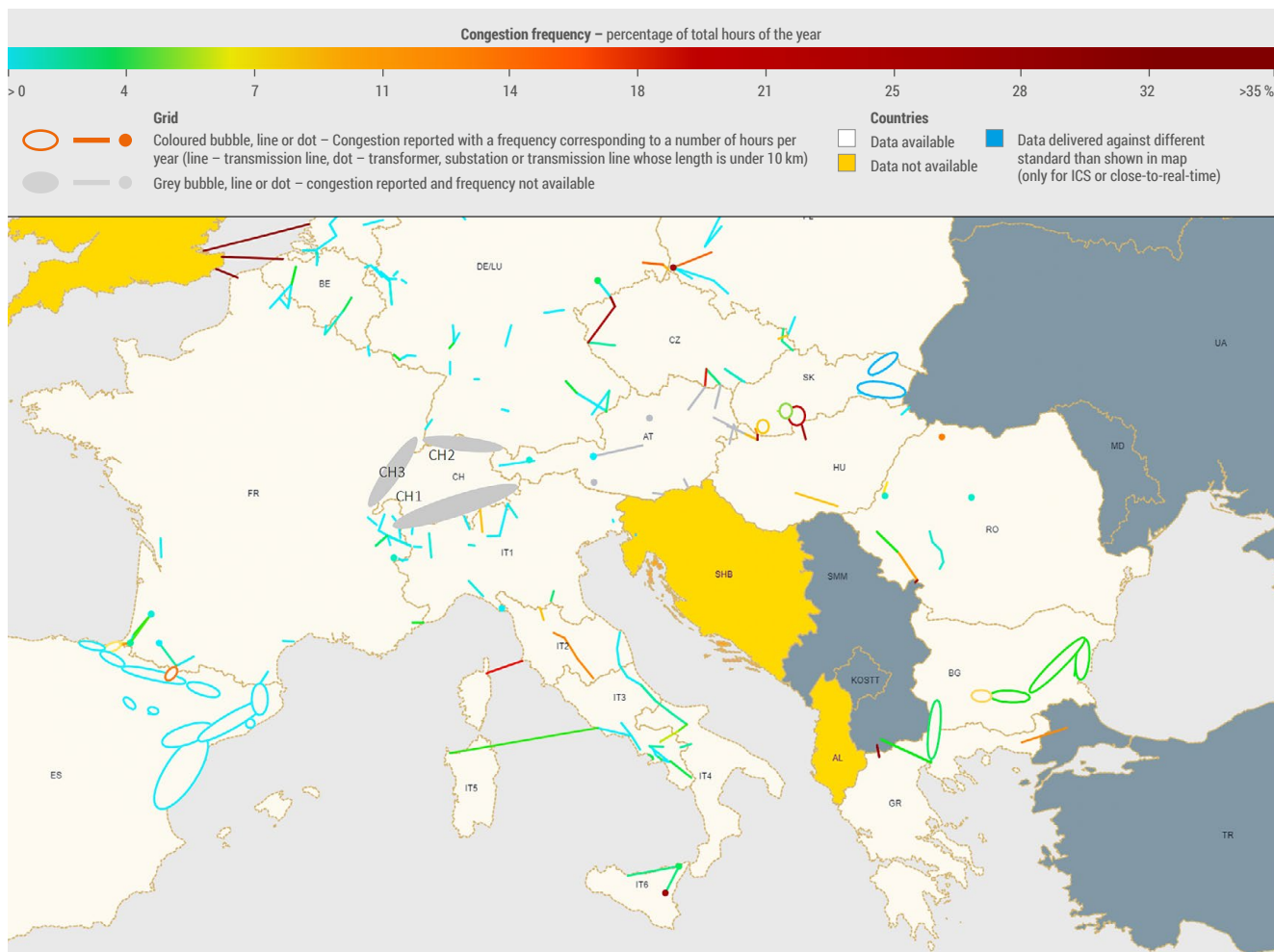
Figure 82: CCDA for 2020 – Balkans and Italy without threshold
