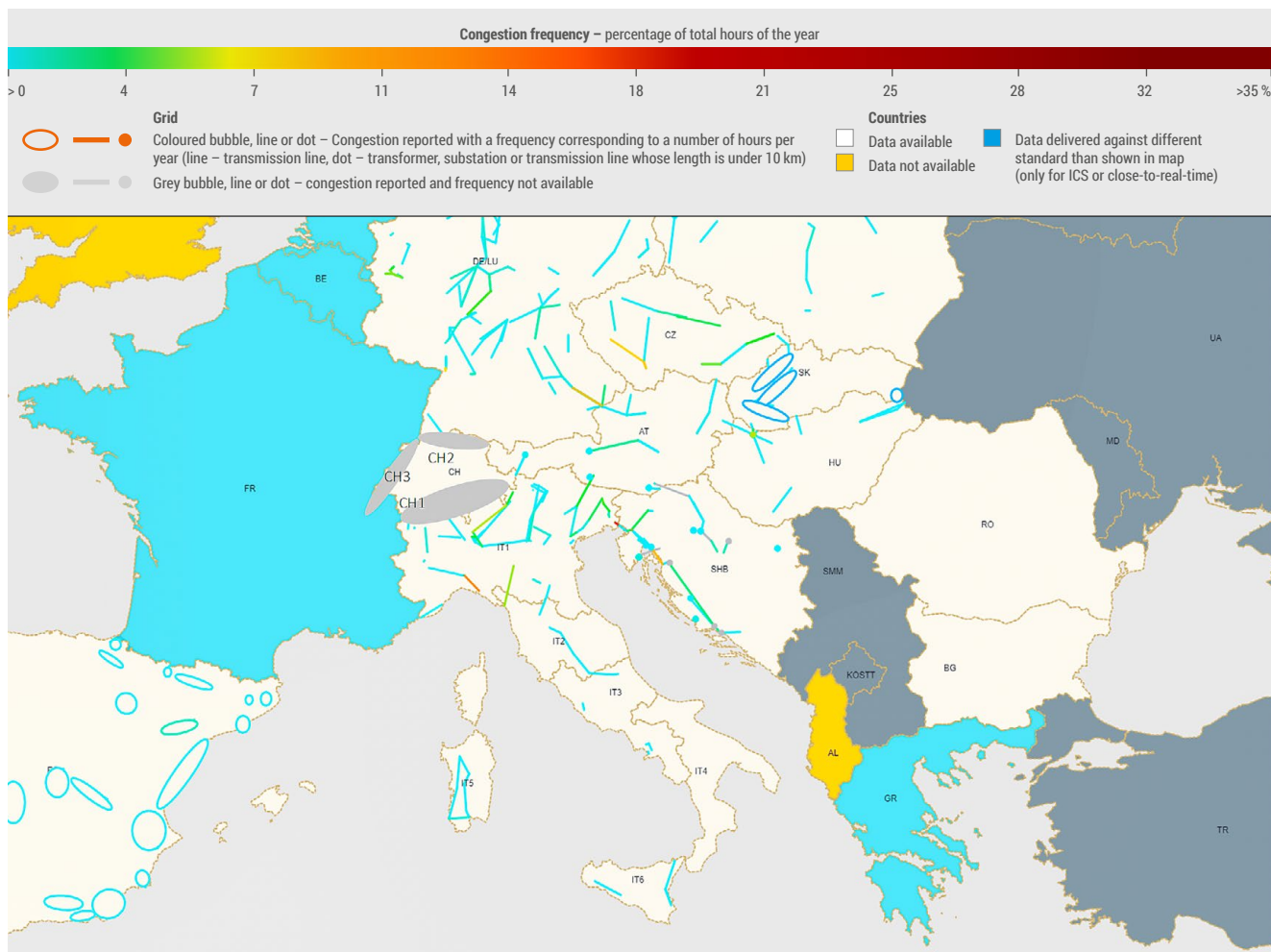
Figure 102: real-time for 2018 – Balkans and Italy without threshold
