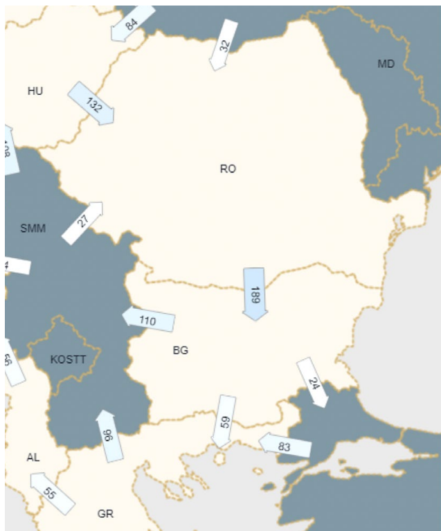
Figure 53: Average PTDF Flow Indicator for 2018 (in MW) – CCR: Southeast Europe (SEE)
