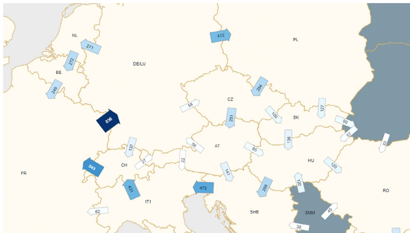
Figure 51: Average PTDF Flow Indicator for 2019 (in MW). CCR: Core and Italy North
