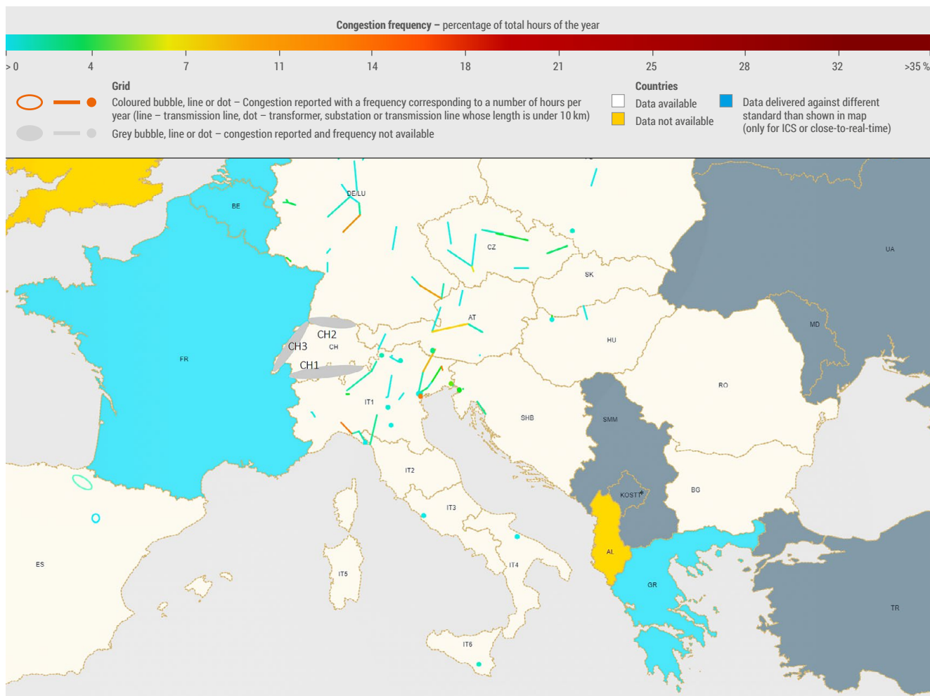
Figure 40: real-time for 2019 – Balkans and Italy
