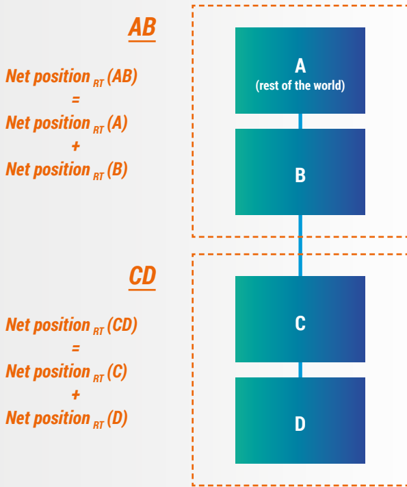
Figure 49: Radially structured network
