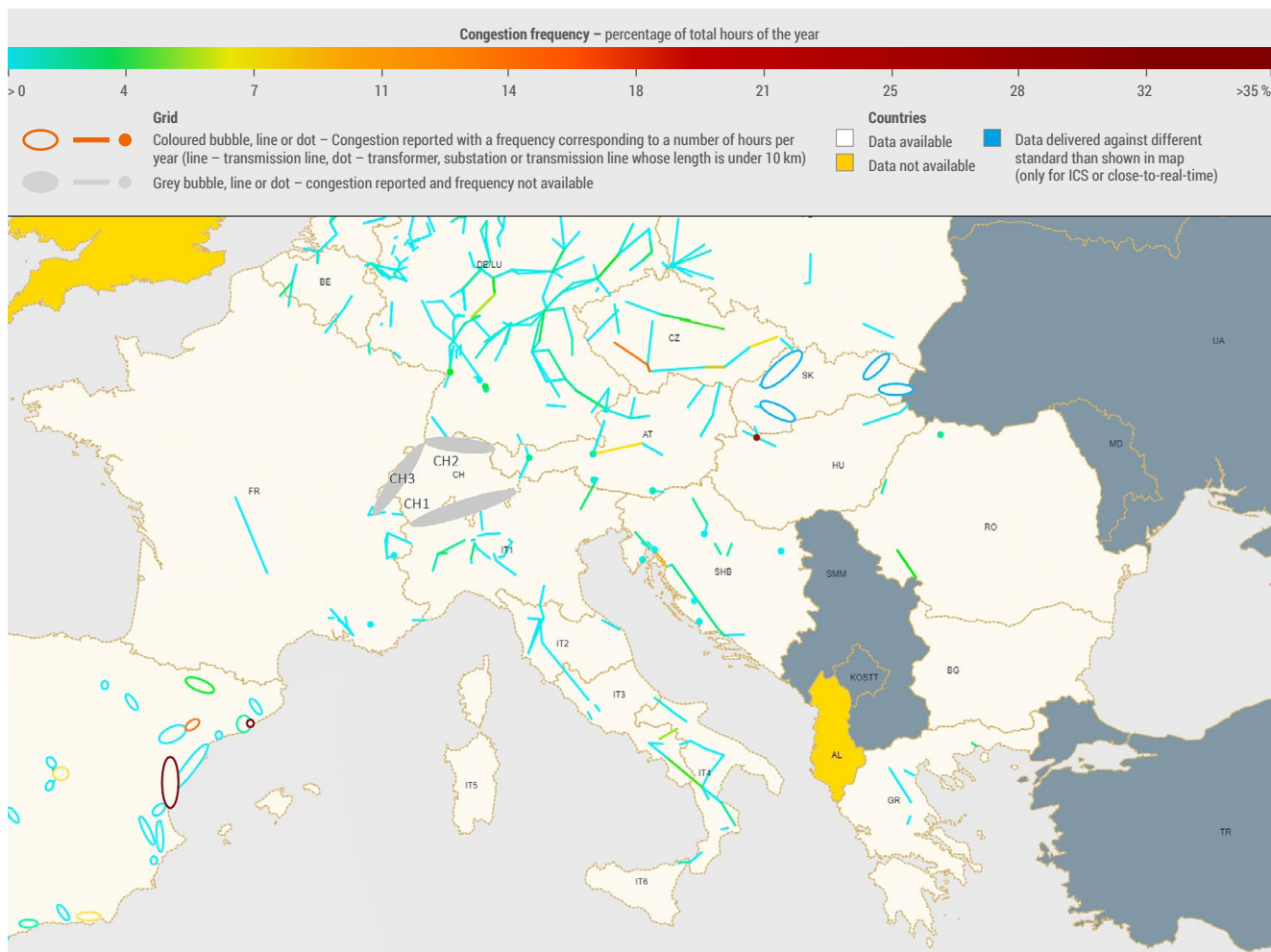
Figure 87: D-1 for 2018 – Balkans and Italy without threshold
