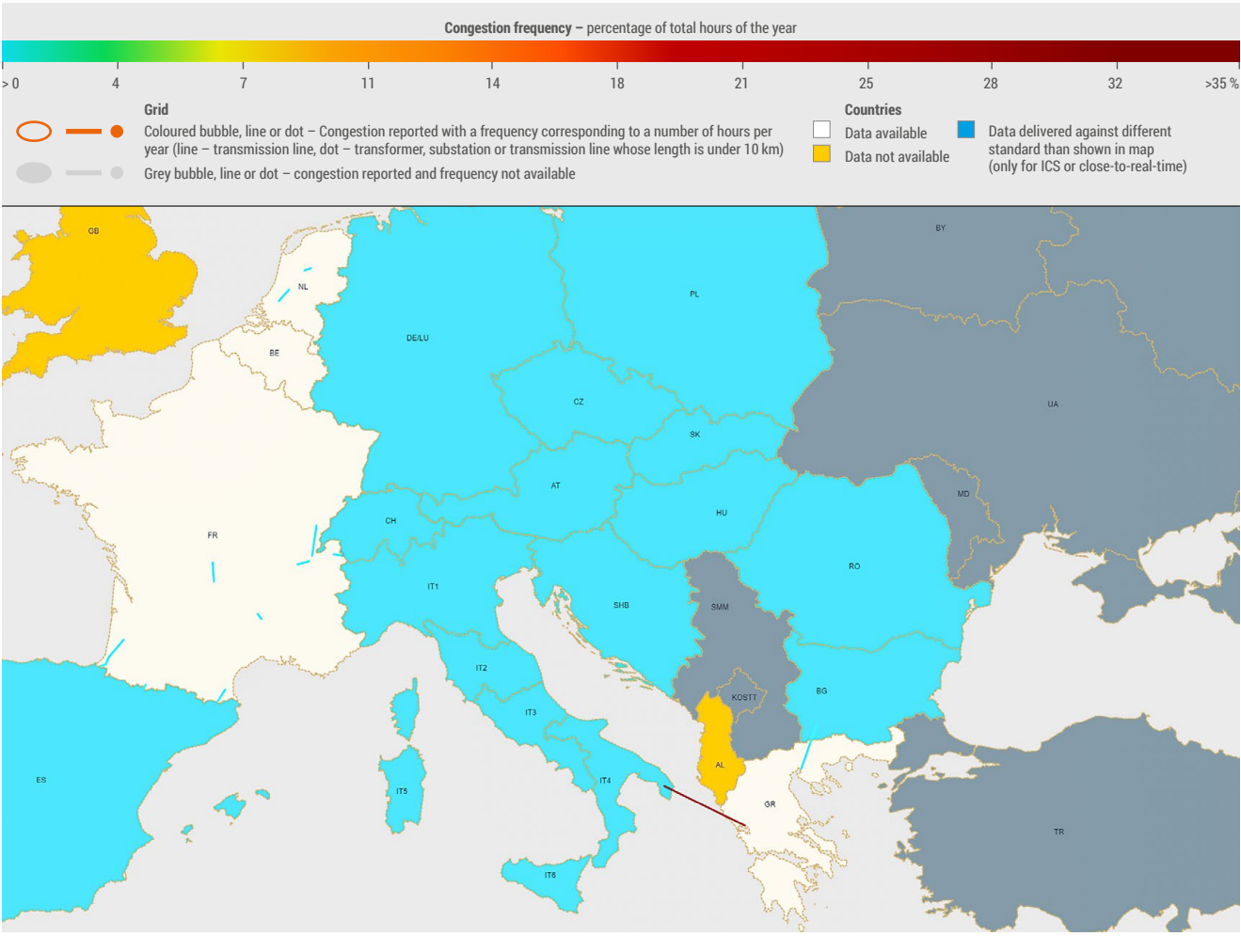
Figure 114: Countries with ICS data, FR, BE, NL and GR only. No threshold
