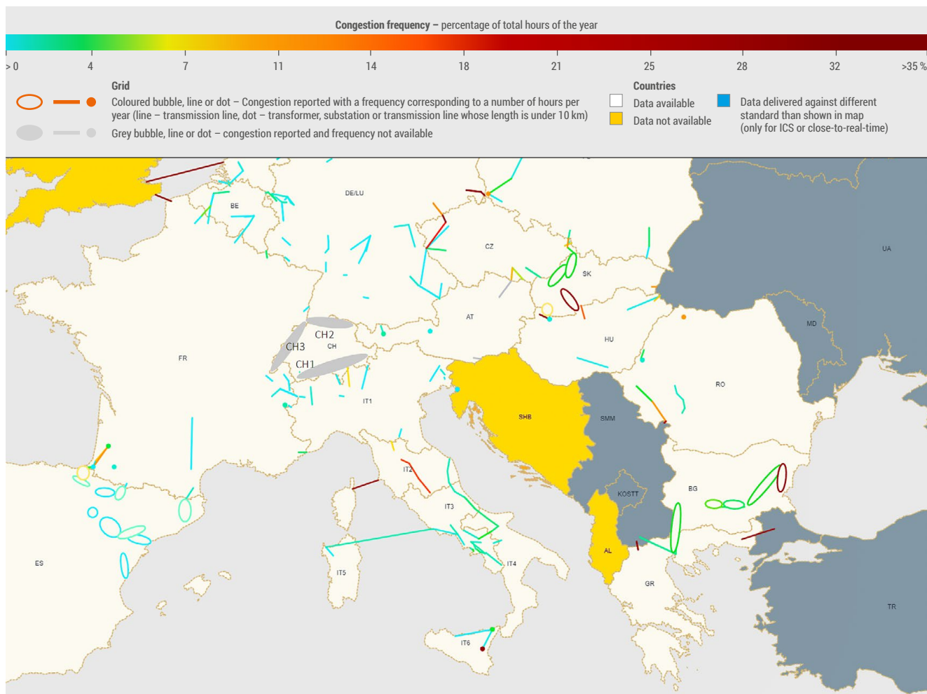
Figure 72: CCDA for 2018 – Balkans and Italy without threshold
