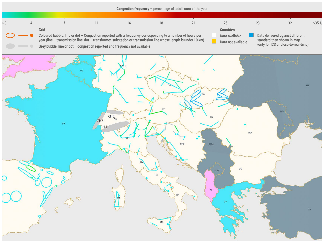
Figure 112: real-time for 2020 – Balkan and Italy without threshold
